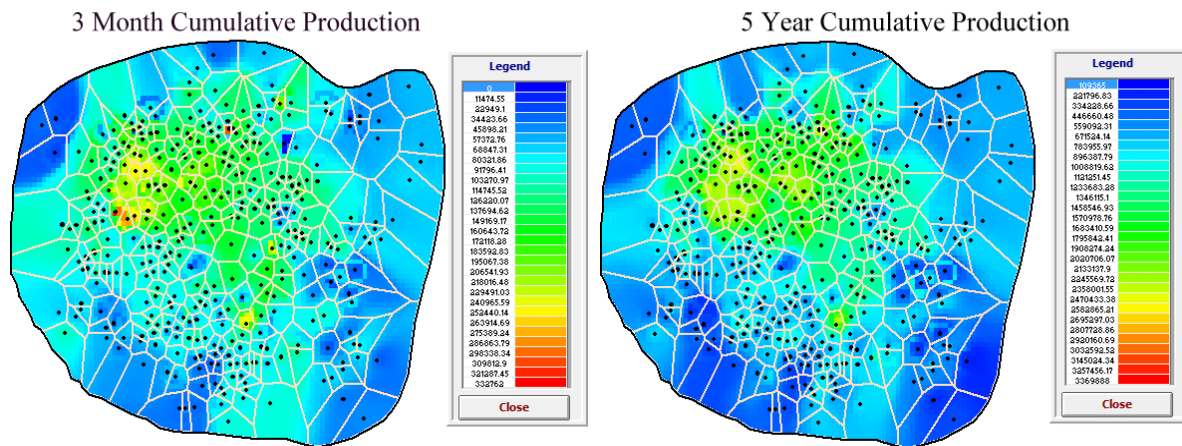
Figure 4. Results of discrete predictive modeling showing the distribution of first 3 months and 5 year cum. production for the entire field.
