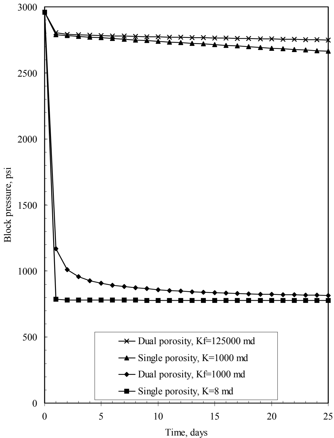
Figure 2- Block pressure history for different runs
