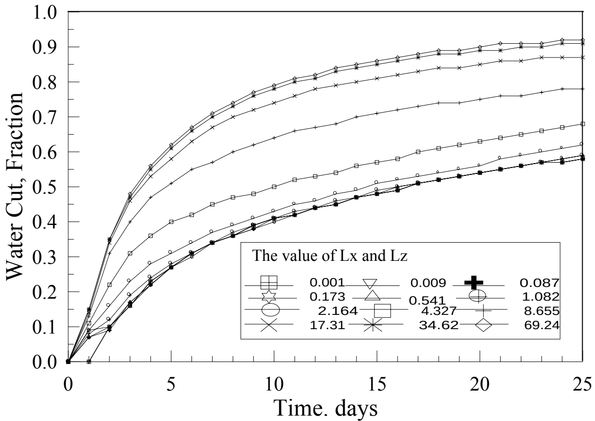
Figure 7- Water cut history for various values of L_s
