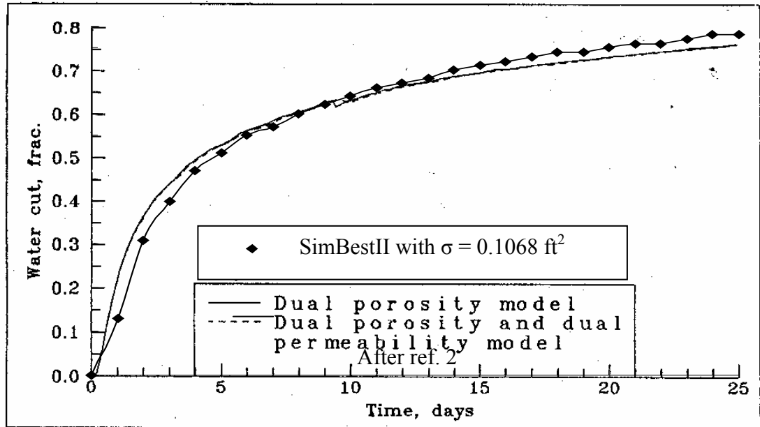
Figure 5– Comparison of water cut history
