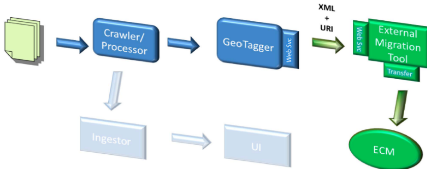
Figure 4: A planned approach to optimizing migration of unstructured data with automated geographic meta-data creation.
